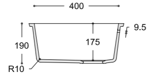
CROSS-SECTION
